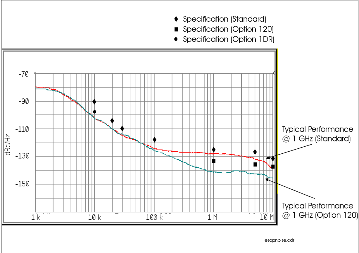
Noise Sidebands Normalized to 1 Hz Versus Offset from Carrier
